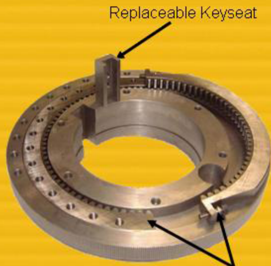
Precision-Split Ring Gear
