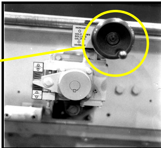
GANG ADJUST HANDWHEEL FOR CALIPER CHANGES
